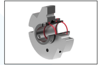
Viking O-Pro Barrier Mechanical Seal
