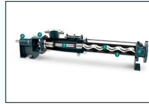
Progressing Cavity Pump
