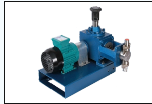
Plunger Type Metering Pump
